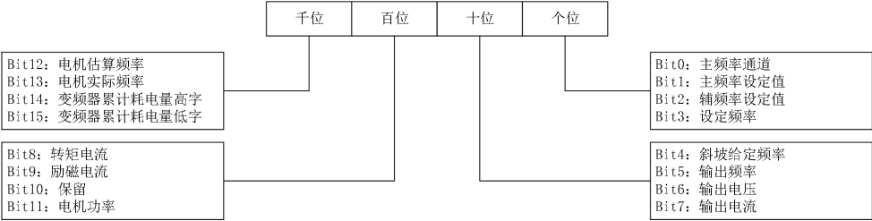
图7-48 LED运行显示参数选择1设定
