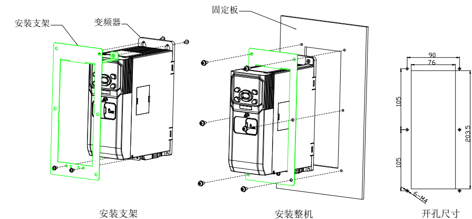
图2-33 MV810-EMBB (适用于0.37~3.7kW)
